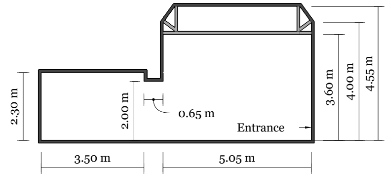
CEILING PLAN
