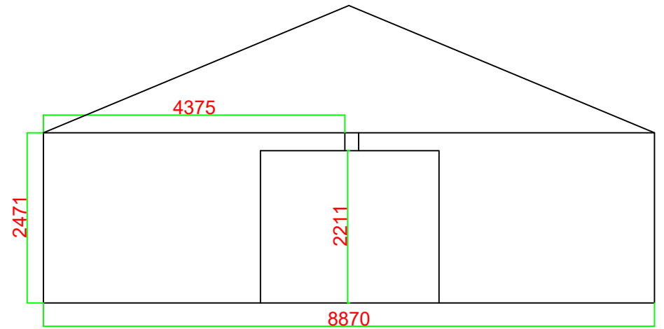
Cross Section of Clubroom
