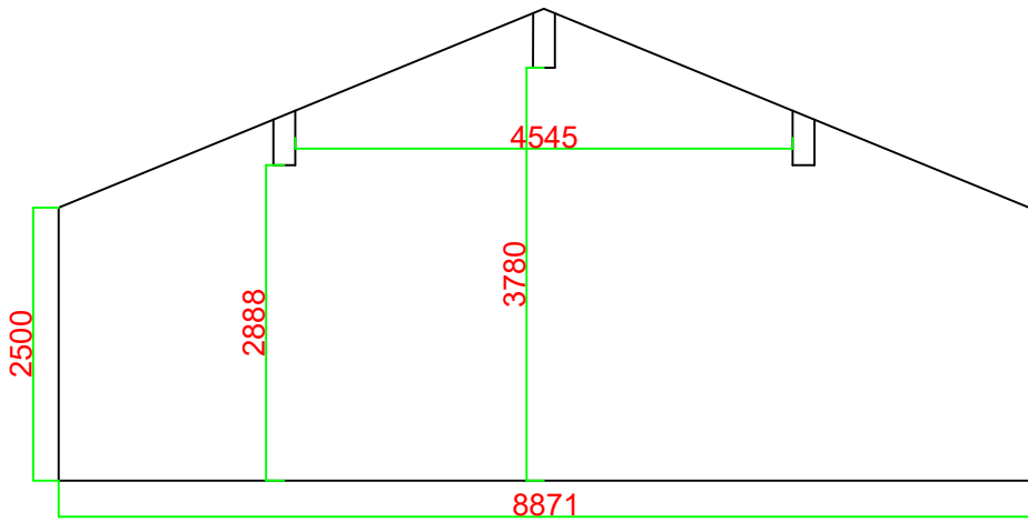
Cross Section of Main Hall
